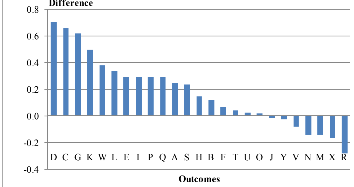
Figure 4.1: Difference Between School-Level R^2 Values Achieved Using the Baseline Test and the “Best” Proficiency Measure for 25 Outcomes
